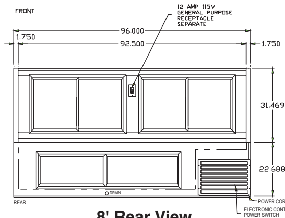
8' Rear View
